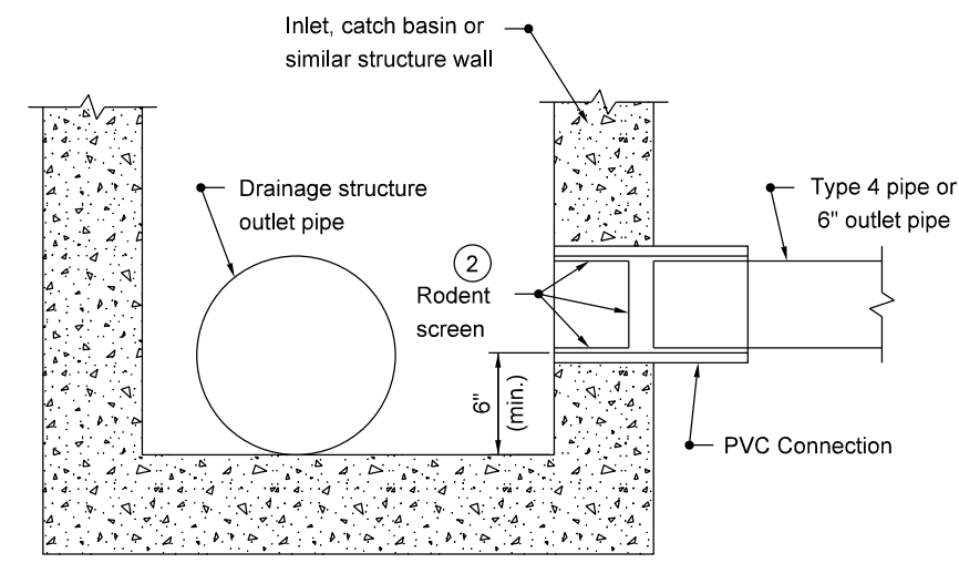
DRAINAGE STRUCTURE OUTLET DETAIL
