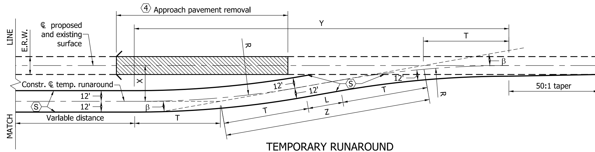
TEMPORARY RUNAROUND
