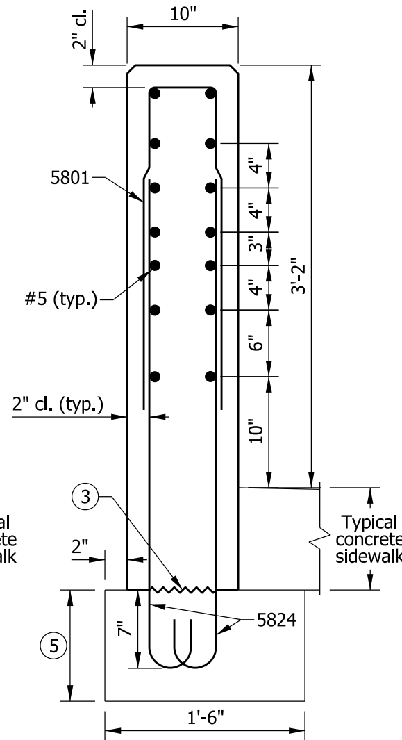
SECTION C-C
