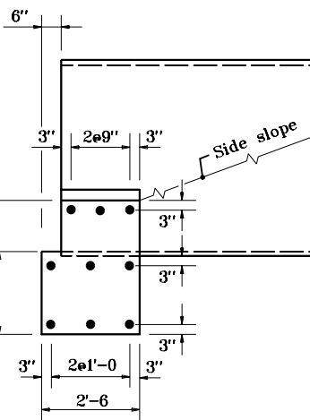
SECTION THROUGH ANCHOR
