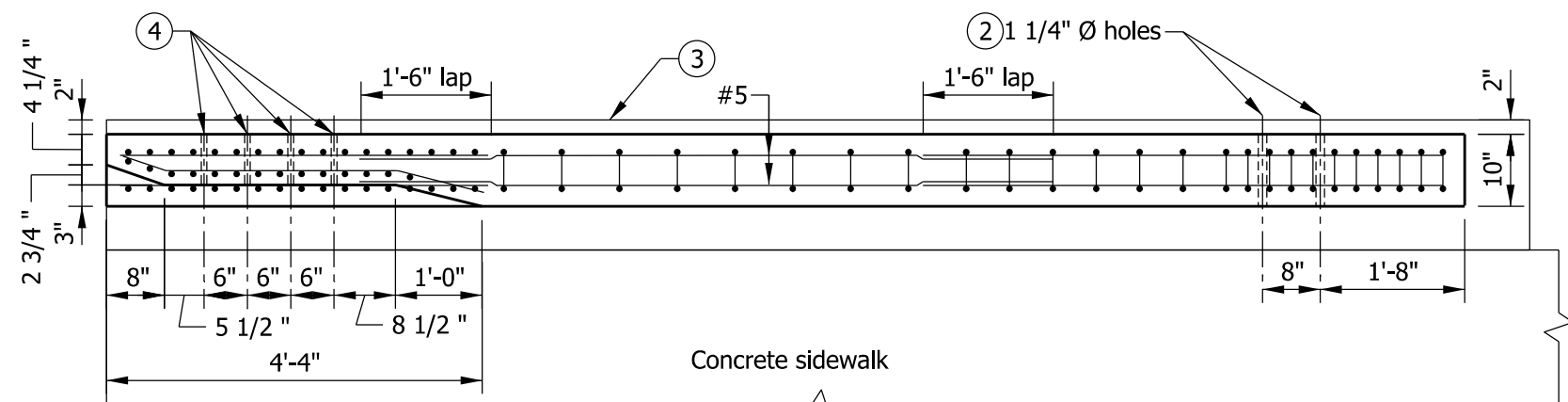
PLAN
