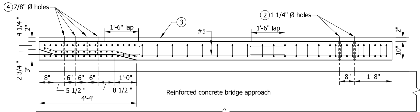
PLAN
