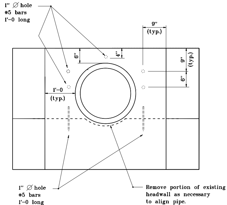
END VIEW
