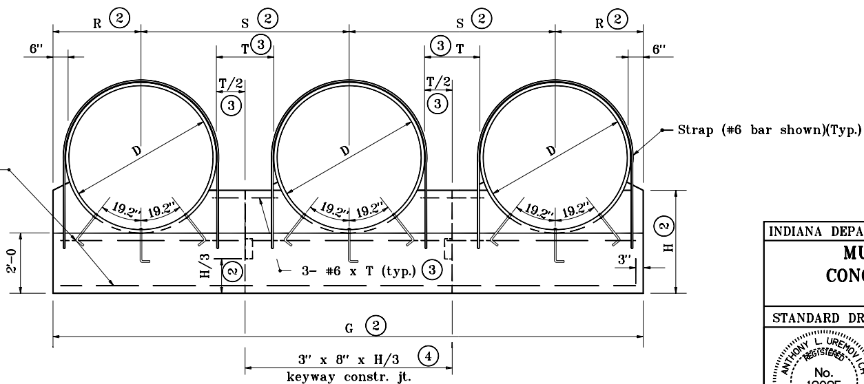
ANCHOR FOR TRIPLE PIPE INSTALLATION FRONT ELEVATION
